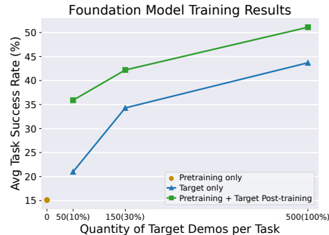
Figure 5: Foundation Model Training Results. Pre-training enables more effective learning of downstream tasks with significant gains in data efficiency.
