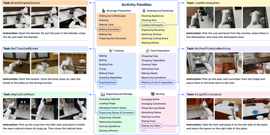
Figure 3: Composite Tasks. RoboCasa365 features 300 composite tasks that involve a sequence of skills. We use large language models to generate a set of high-level activities, and for each activity, a set of task blueprints. There are 6 activity families (high-level categories) spanning 60 activities, which organize composite tasks based on shared functional and semantic structure. Representative tasks are shown for selected activities.
